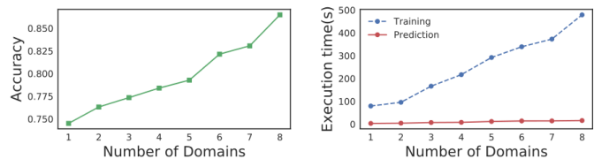
Fig. 4. Accy. &amp; Exec. Time vs. # of Domains
