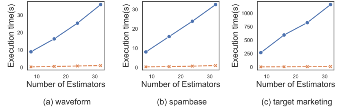
Fig. 6. Prediction Time vs. Number of Estimators
