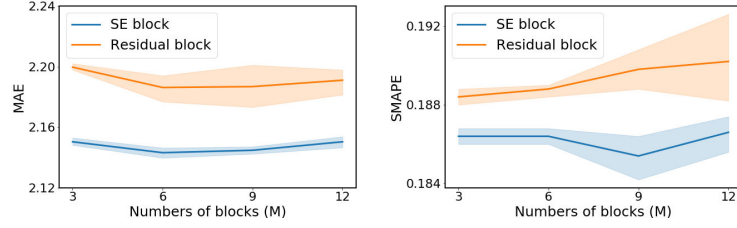
Fig. 7. SE vs. residual block over P1, where the shade area is the standard deviation.
